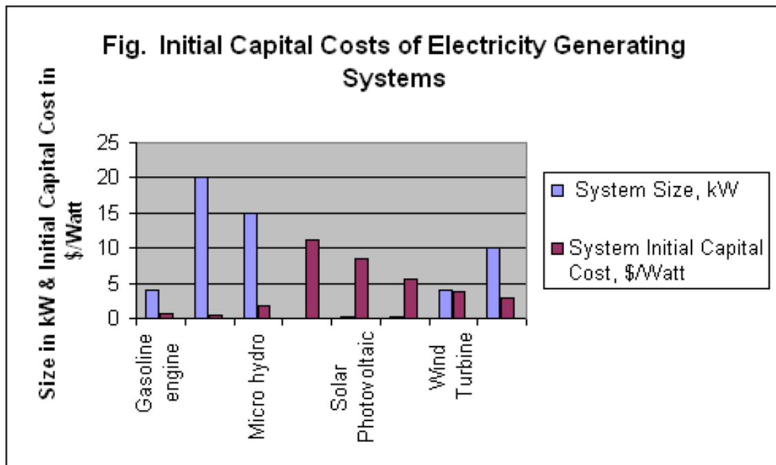
Fig. 2.1.3 Initial capital costs of electricity generating systems
